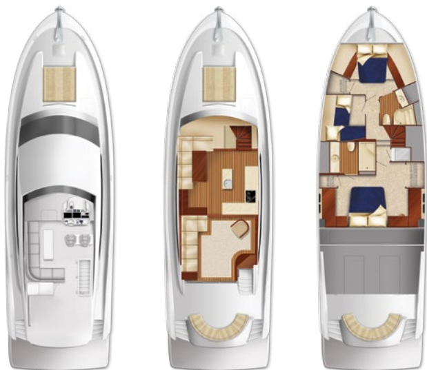
FLYBRIDGE ARRANGEMENT
