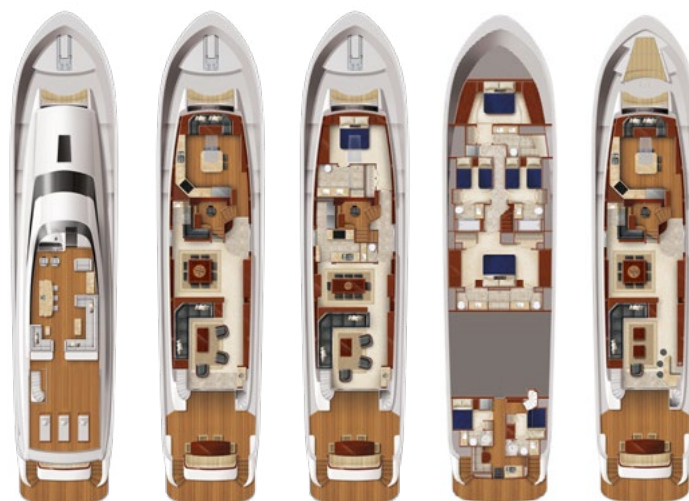
FLYBRIDGE ARRANGEMENT
